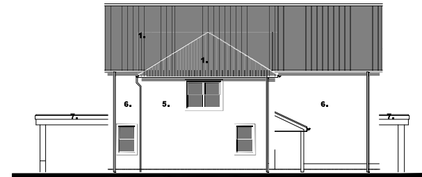
SIDE ELEVATION 1
